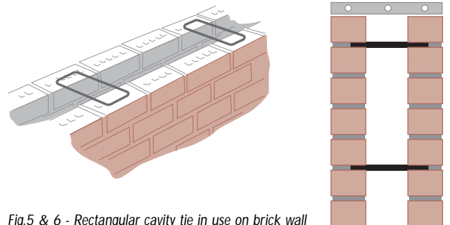
Fig.5 & 6 - Rectangular cavity tie in use on brick wall
