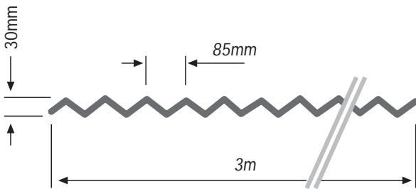
Fig.3 - Snake wire dimensions
