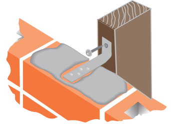
Fig.1 Supplied with screw fixings for wood or steel
