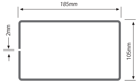
Fig.4 - Rectangular cavity tie dimensions
