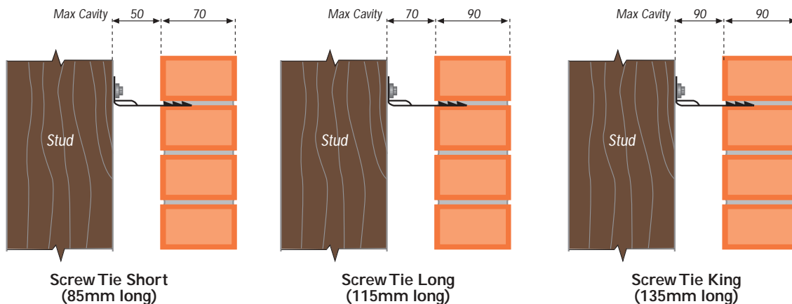
Fig.2 Ties available in 3 lengths
