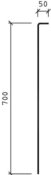
Bricklock NET dropper
