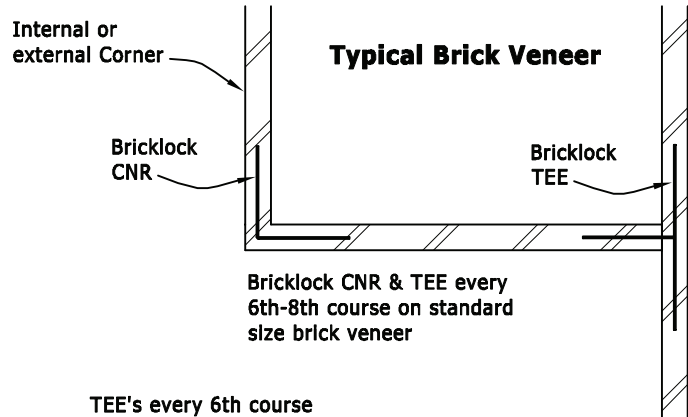
Bricklock CNR
