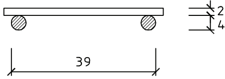
Bricklock Profile (Scale F.S.)
